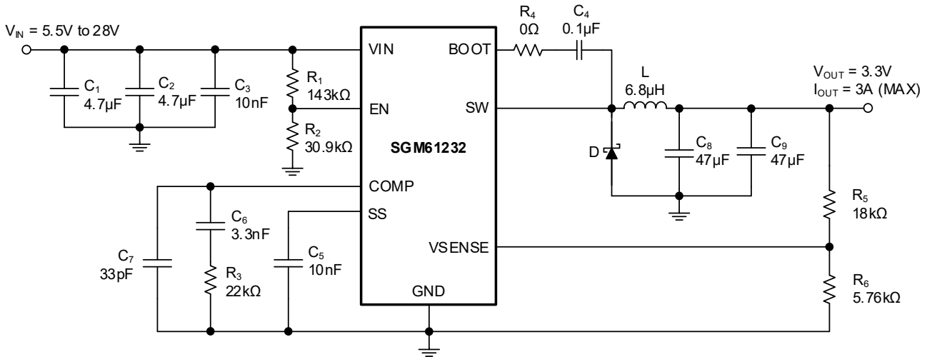
Figure 4. SGM61232 Typical Application Circuit
