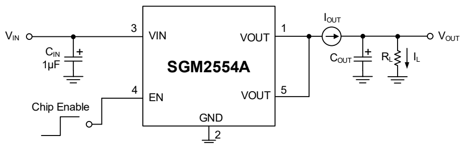
Test Circuit 1
