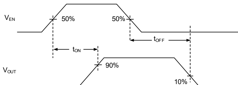
Switch Turn-On or Turn-Off Delay Time
