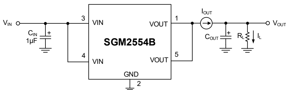
Test Circuit 2
