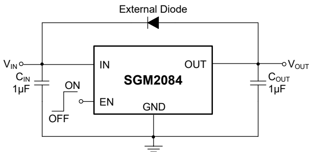
Figure 5. Reverse Protection Reference Design
