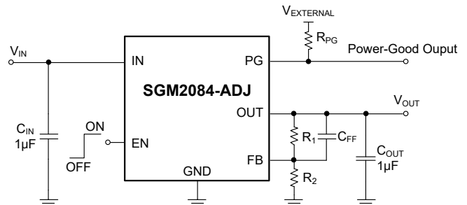
Figure 4. Adjustable Output Voltage Application
