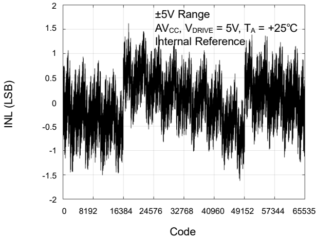
SGM51652S8 Typical INL, ±5V Range
