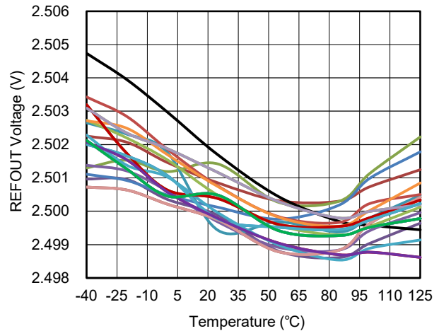
REFOUT Voltage vs. Temperature
