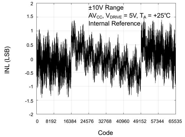
SGM51652S8 Typical INL, ±10V Range
