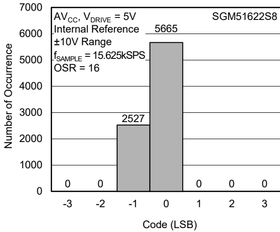
Figure 21. Histogram of Codes (OS × 16)
