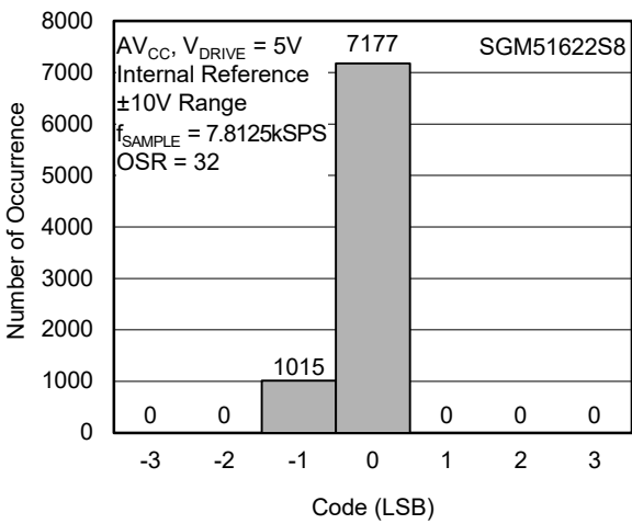
Figure 22. Histogram of Codes (OS × 32)
