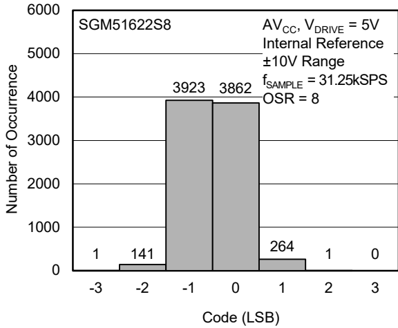
Figure 20. Histogram of Codes (OS × 8)
