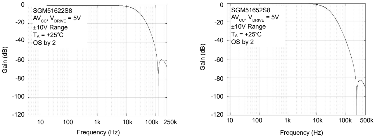
Figure 24. Digital Filter Response for OS 2
