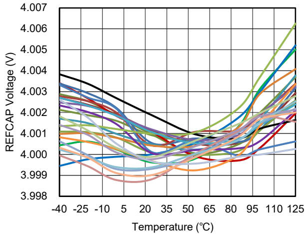
REFCAP Voltage vs. Temperature
