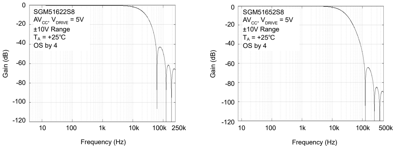
Figure 25. Digital Filter Response for OS 4
