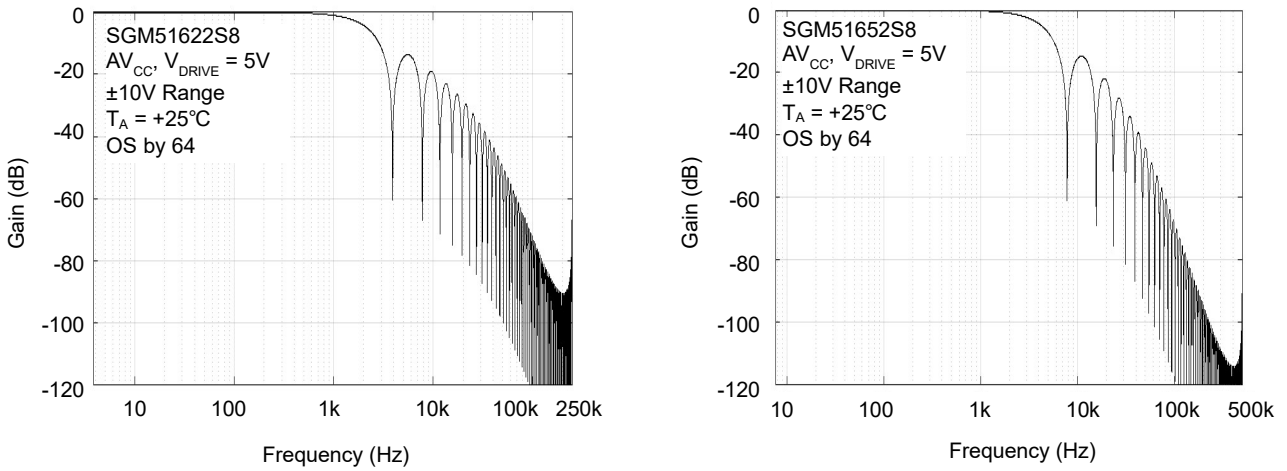
Figure 29. Digital Filter Response for OS 64
