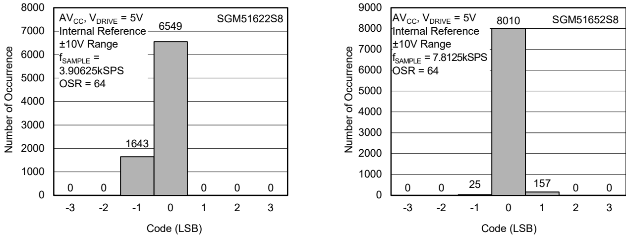
Figure 23. Histogram of Codes (OS × 64)
