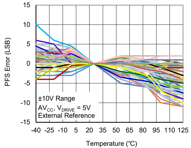
PFS Error vs. Temperature
