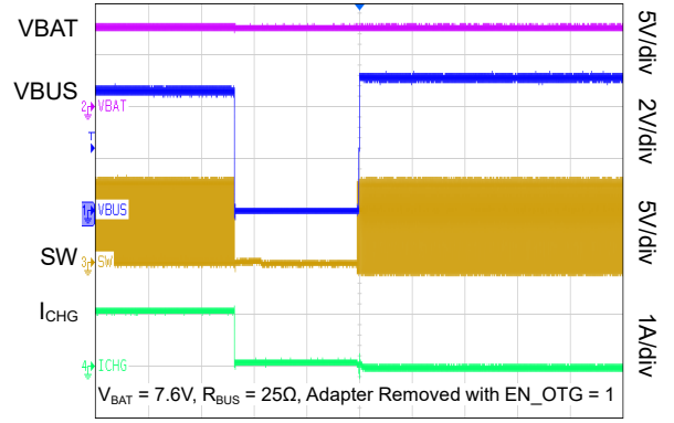
Time (10ms/div)
