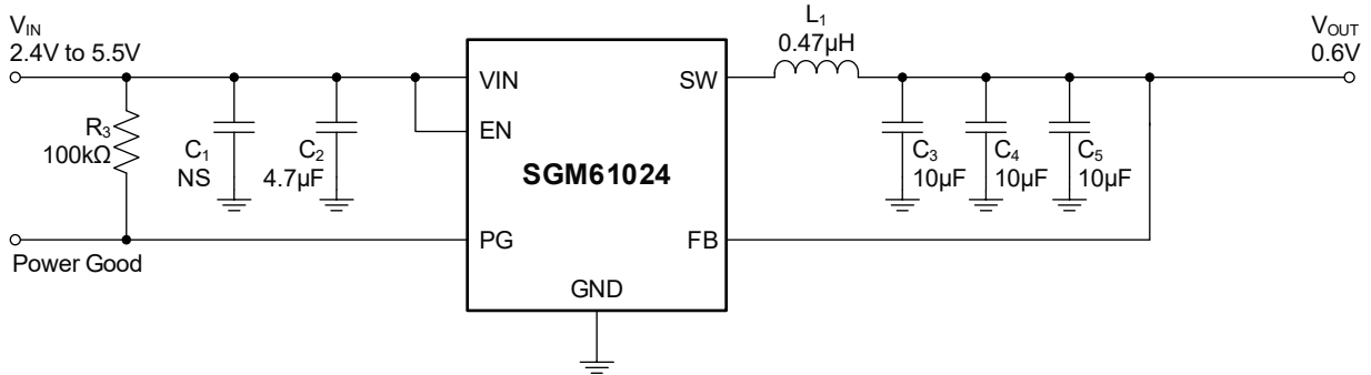
Figure 5. 0.6V Output Voltage Application of SGM61024
