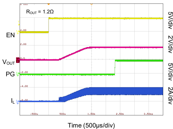
Startup with Load (SGM61024A)
