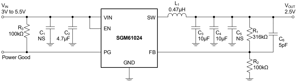
Figure 7. 2.5V Output Voltage Application of SGM61024
