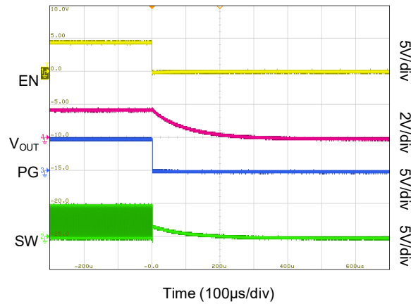
Disable with No Load (SGM61024B)
