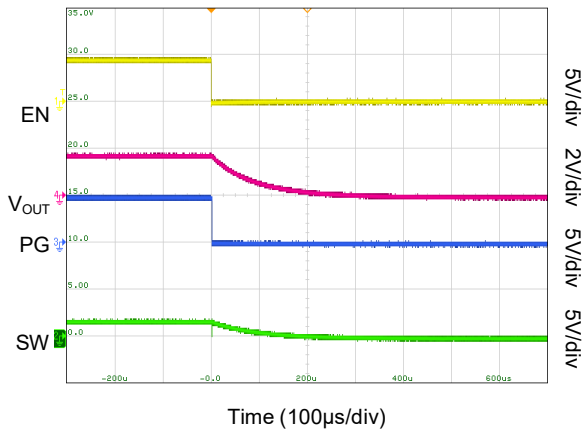
Disable with No Load (SGM61024A)
