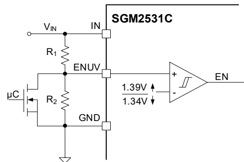
Figure 8. Shutdown Control
