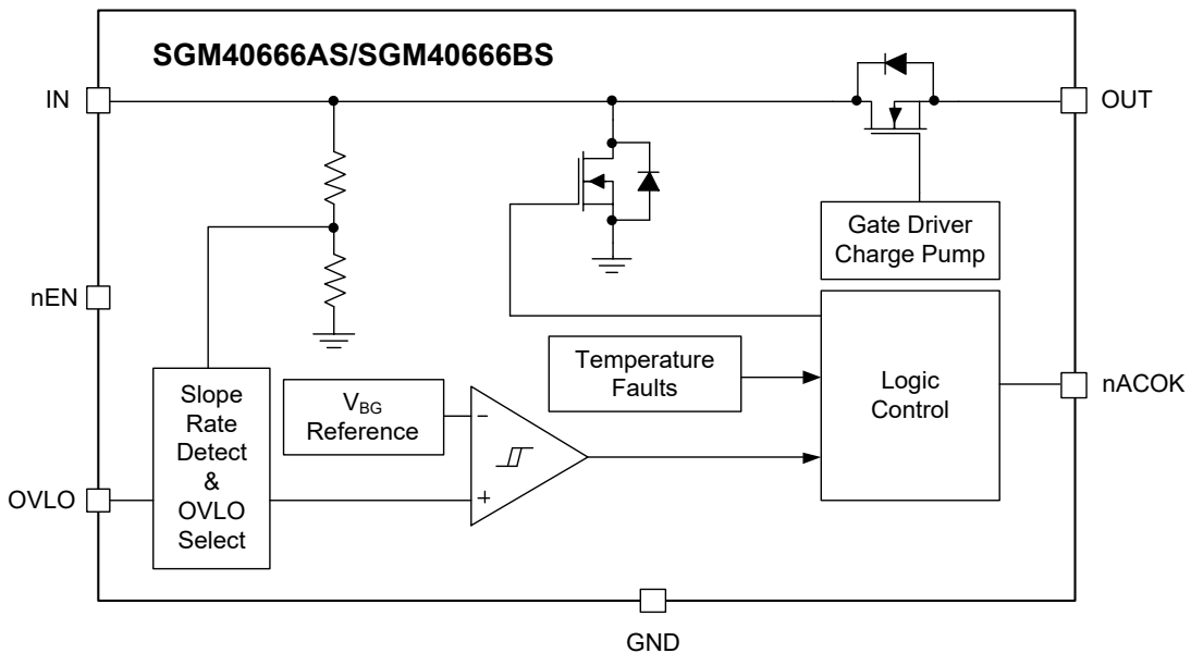
Figure 2. Block Diagram
