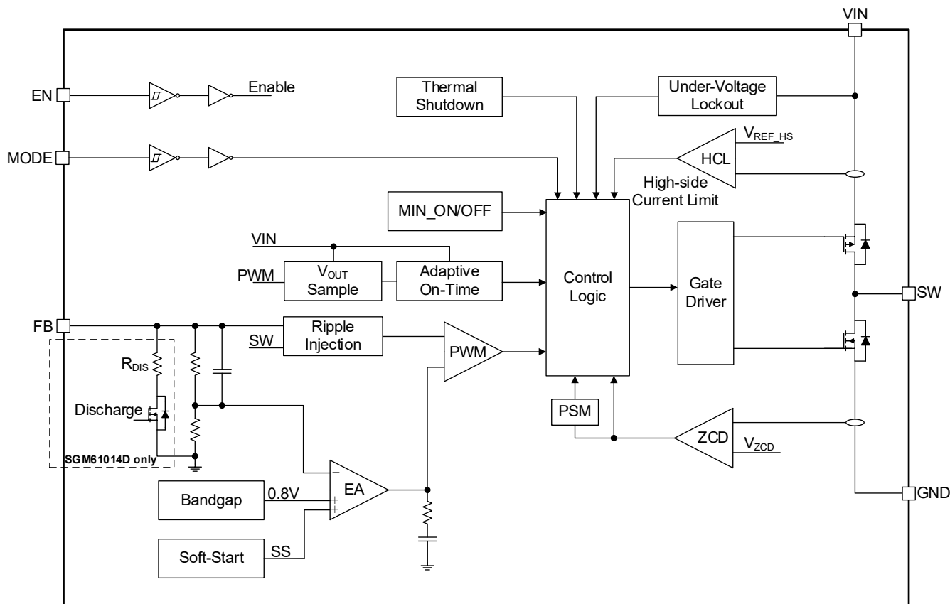
Figure 2. Block Diagram
