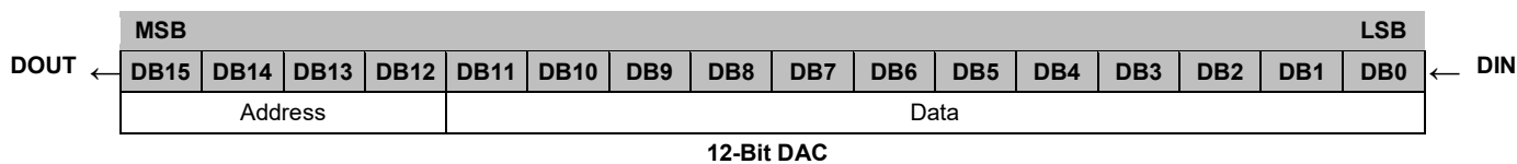
12-Bit DAC Figure 1. Serial Data
