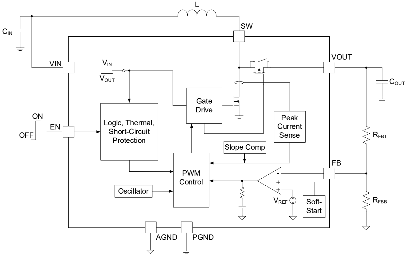
Figure 2. Block Diagram
