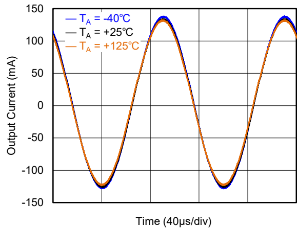
Figure 7. Output Current of Resolver Excitation Circuit
