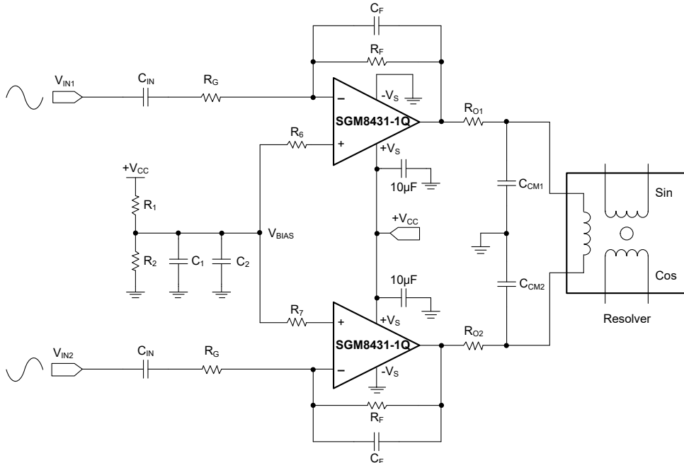
Figure 3. Simplified Resolver Excitation Circuit without SGM8212-1Q
