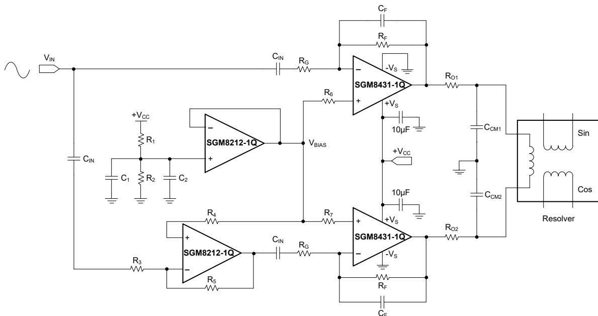
Figure 1. Resolver Excitation Circuit
