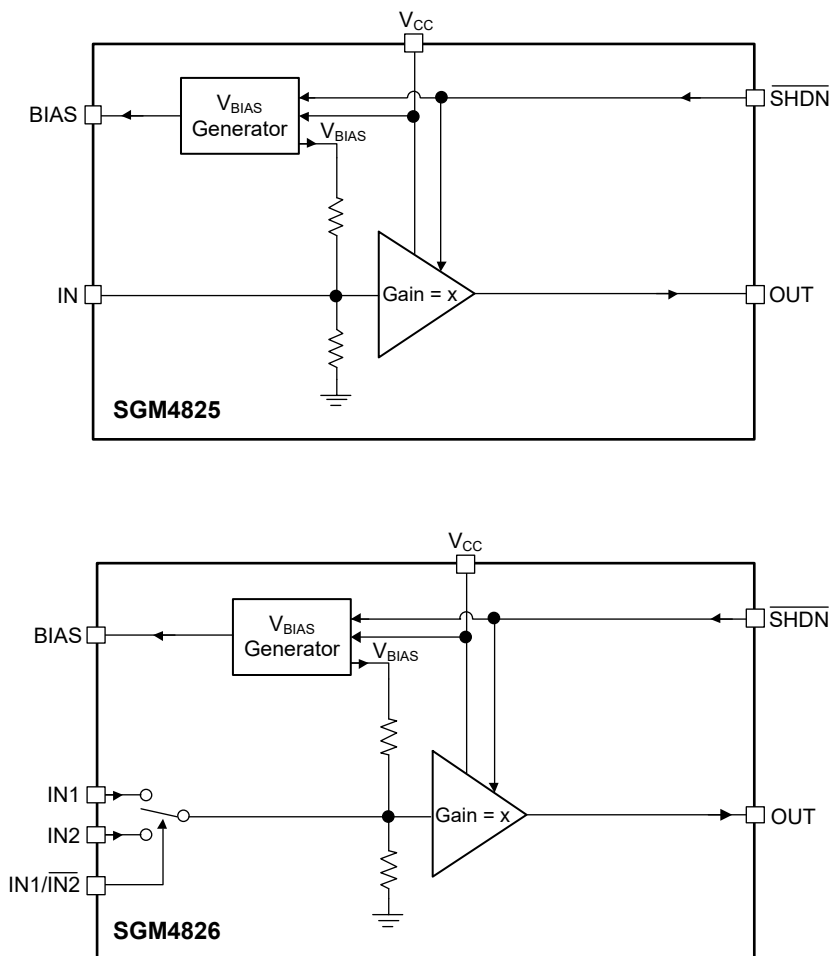
Figure 1. Block Diagram
