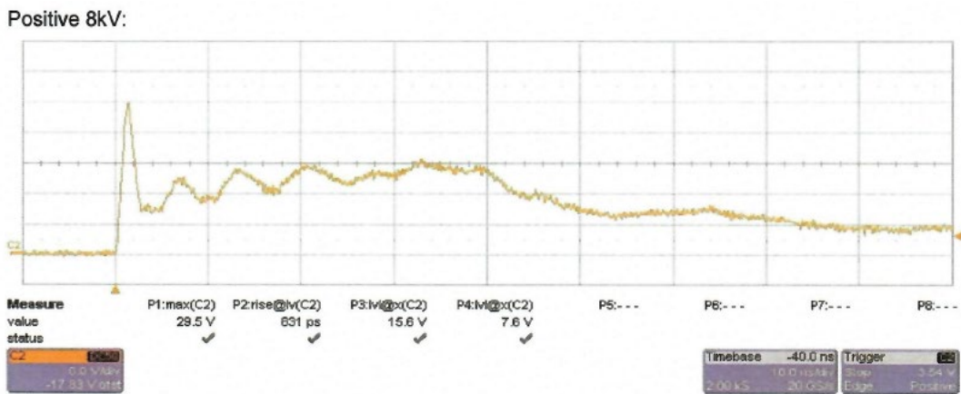
Figure 1. Typical Pulses ESD 8kV Contact per IEC 61000-4-2
