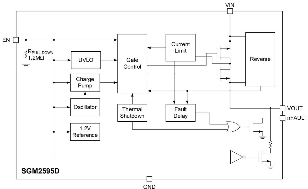
Figure 2. Block Diagram
