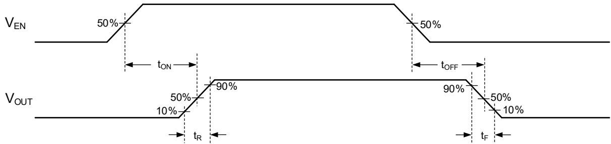
Figure 3. Switch Turn-On Time and Turn-Off Times
