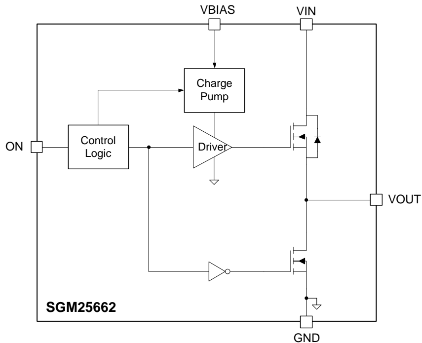
Figure 4. Block Diagram
