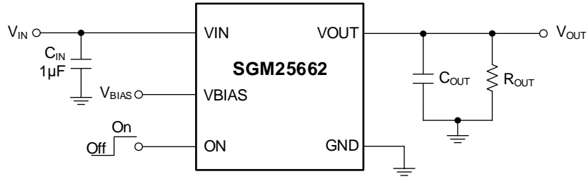
Figure 2. Test Circuit
