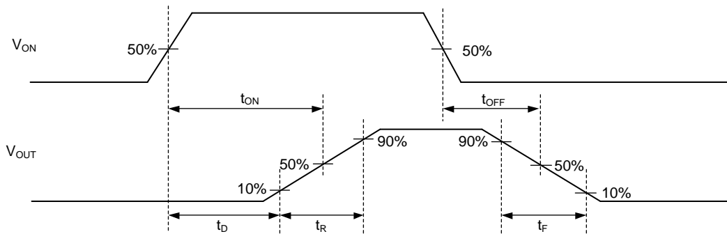
Figure 3. Turn-On and Turn-Off Waveforms
