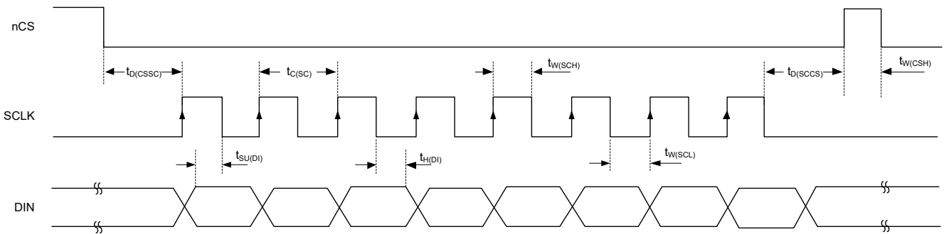
Figure 1. Serial Interface Timing Diagram
