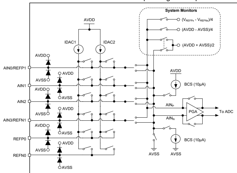
Figure 5. Analog Input Multiplexer
