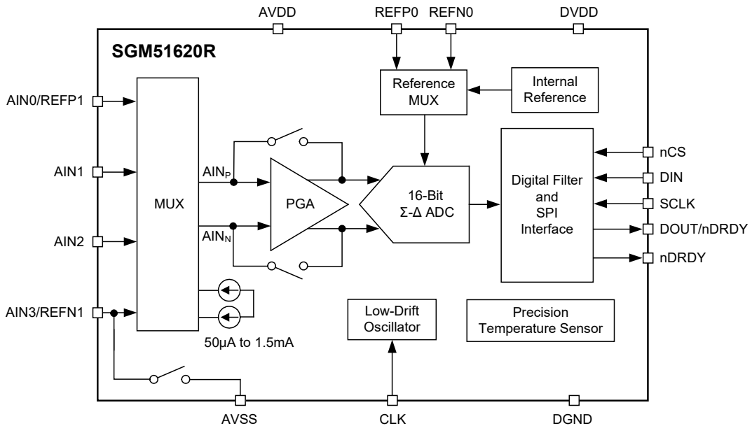
Figure 4. Block Diagram
