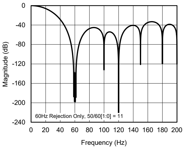
Figure 15. Filter Response (DR = 20SPS)
