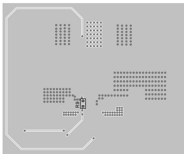
Figure 15. Bottom Layer
