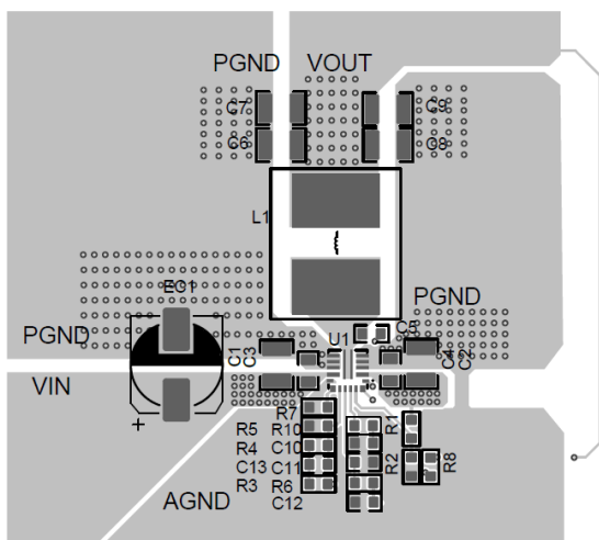
Figure 12. Top Layer
