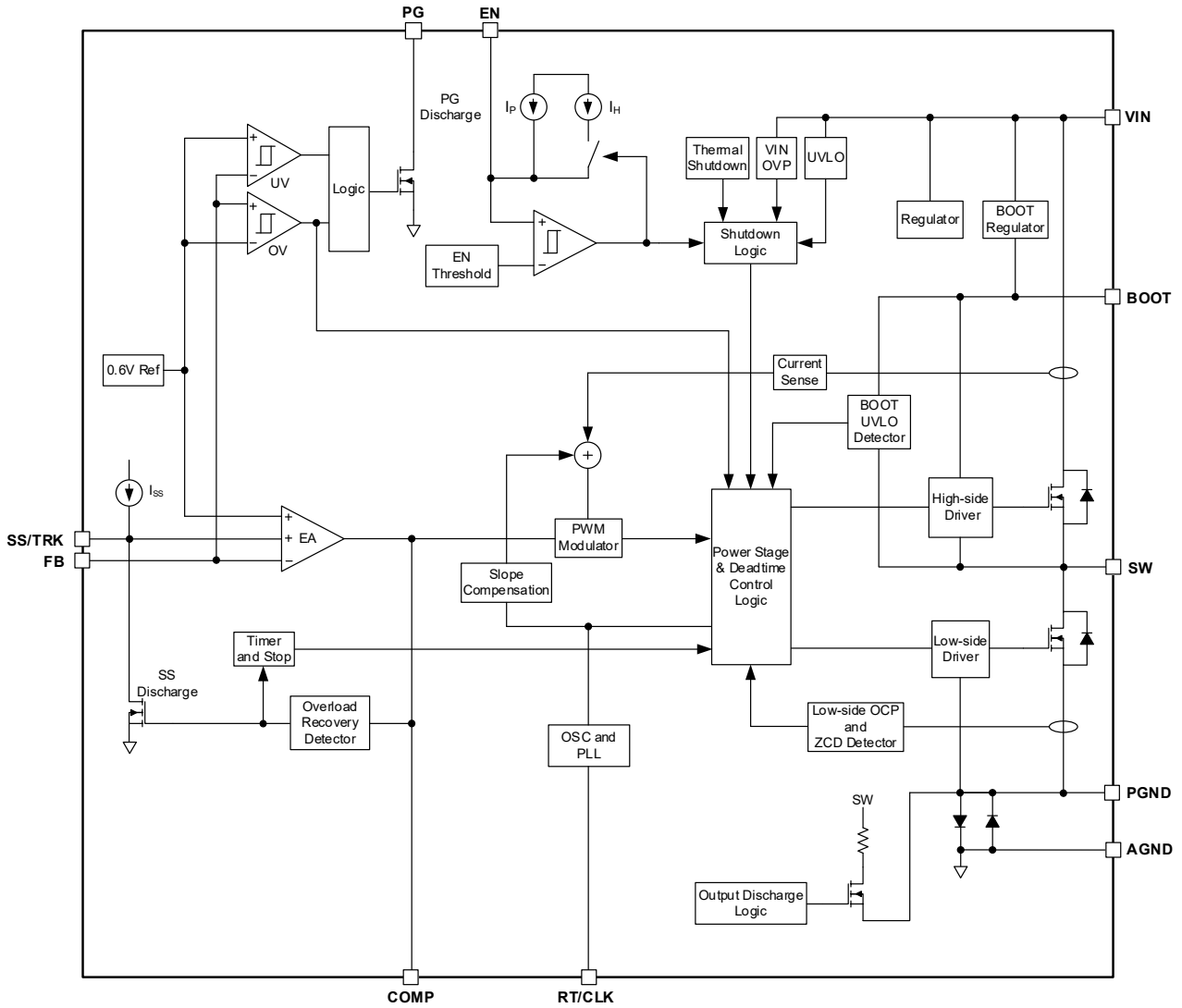
Figure 2. Block Diagram
