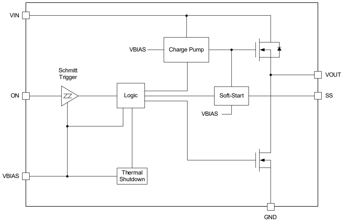
Figure 3. Block Diagram
