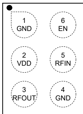
UTDFN-1.1×0.7-6L
