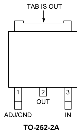
SGM2240xQ (TOP VIEW)
