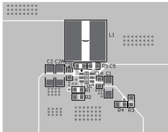
Figure 6. Top Layer
