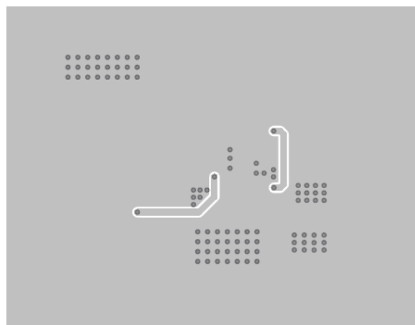
Figure 7. Bottom Layer
