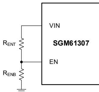
Figure 4. System UVLO by Enable Divider
