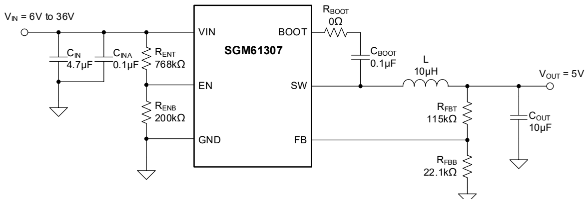
Figure 5. Application Circuit
