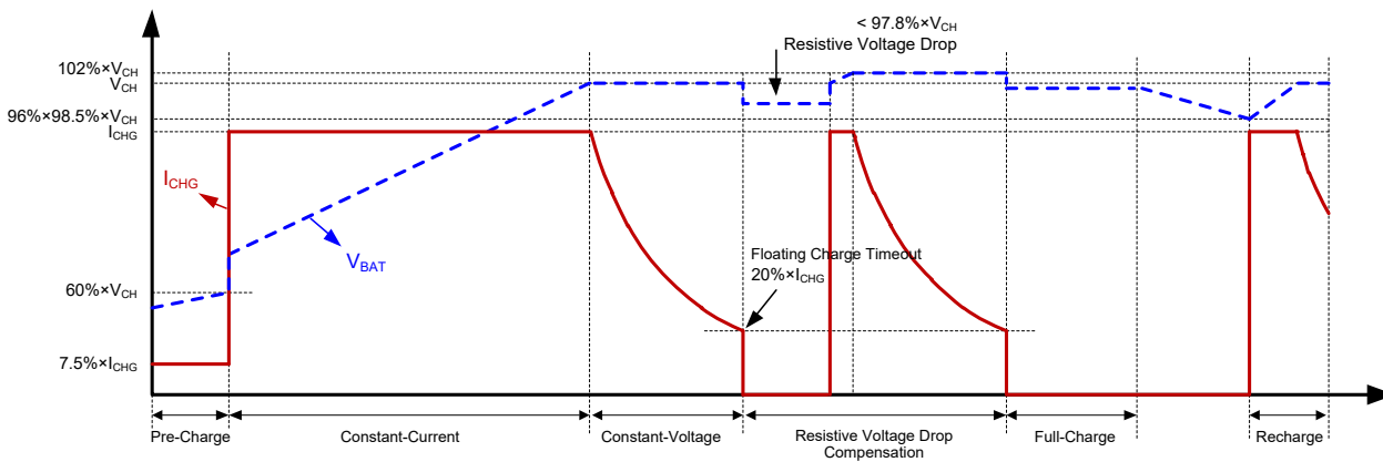
Figure 5. Charge Profile (Resistive Voltage Drop > 2.2\% \times V_{CH}</math>)
