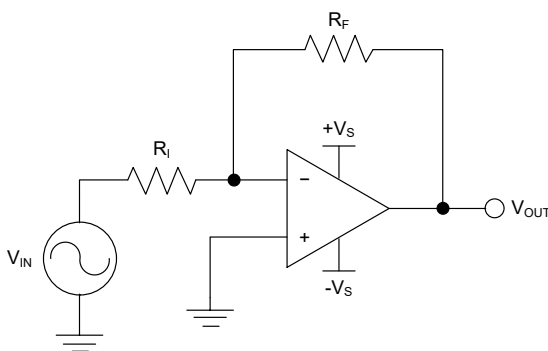
Figure 1. Application Schematic
