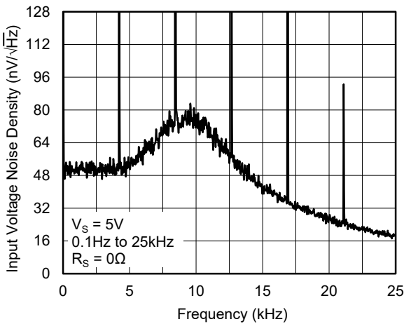
Input Voltage Noise Density vs. Frequency
