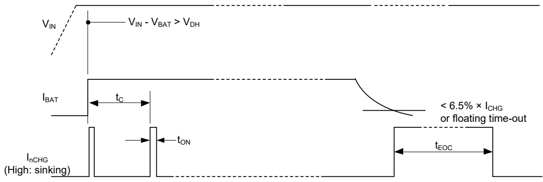
Figure 3. nCHG Driving Timing Diagram
