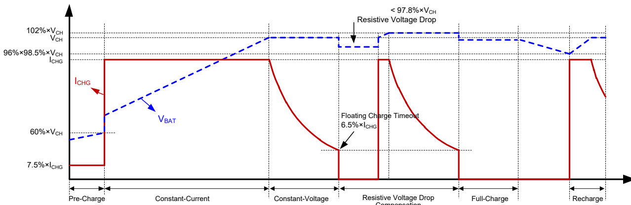
Figure 5. Charge Profile (Resistive Voltage Drop > 2.2\% \times V_{CH} )
