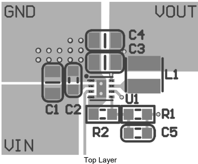
Figure 10. PCB Layout
