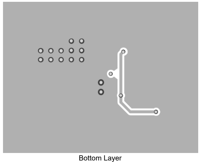
Figure 10. PCB Layout
